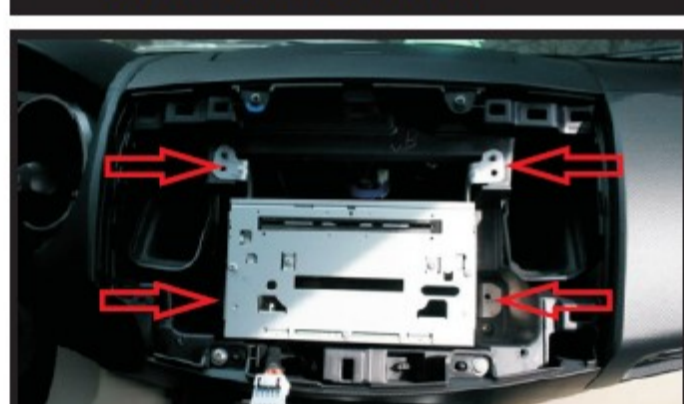
5. Pry the screws of the CD player.
