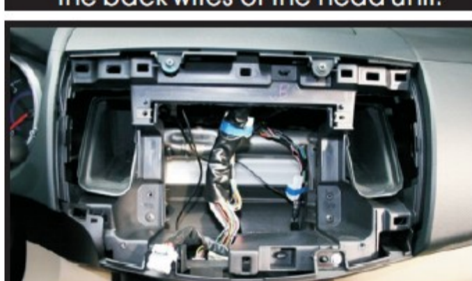
6. Take out the console of head unit.
